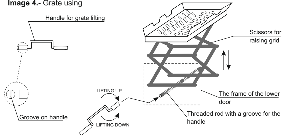
Image 4.- Grate using
