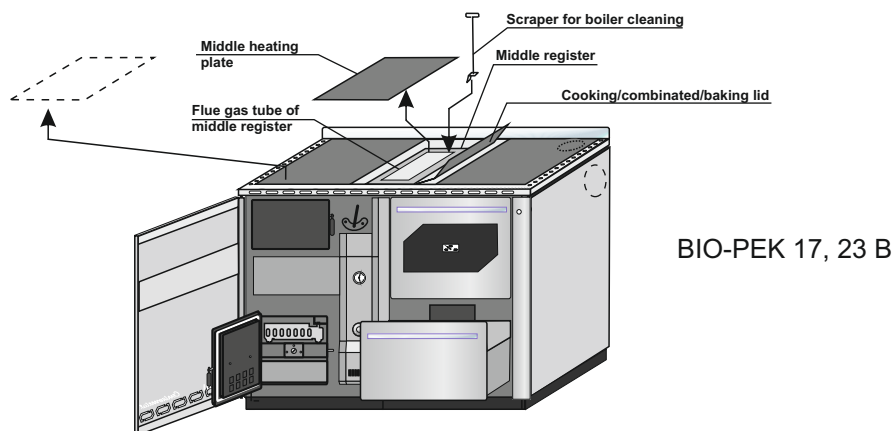
Image 8. Exchange surfaces cleaning - BIO-PEK B-D (applies to BIO-PEK B - L)
