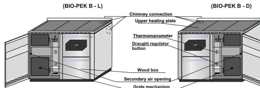
Image 9. Basic parts
