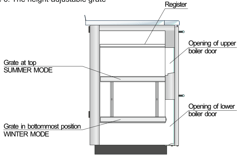
Image 6. The height-adjustable grate
