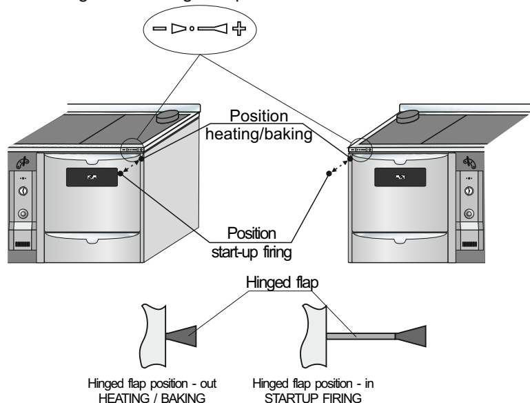
Image 3. Handling with the hinged flap of the BIO-PEK B
