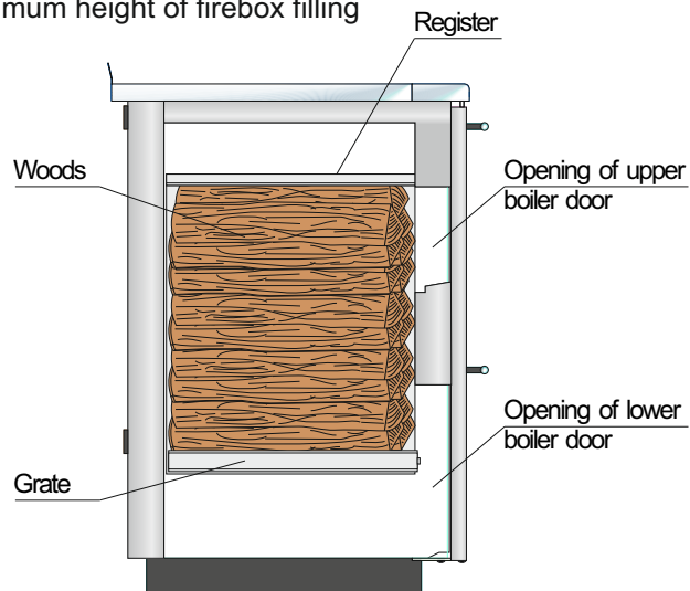
Image 2. Maximum height of firebox filling
