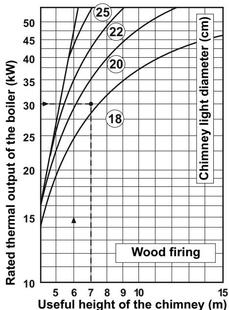
Image 1. Dimensioning of the chimney for BIO-PEK B
